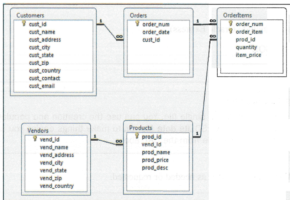
FIGURE A.1 Sample tables relationship diagram
